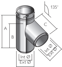
135° Tee
